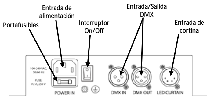
Panel Superior
